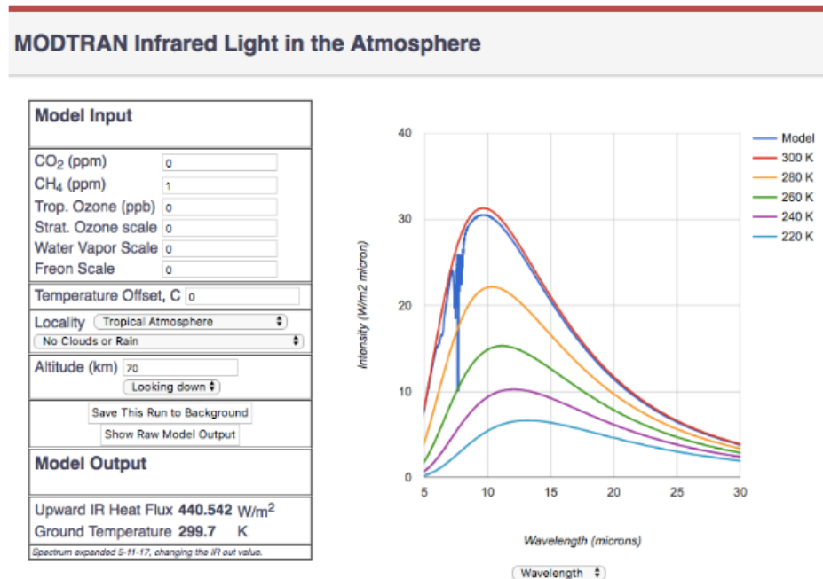
Figure 1: https://climatemodels.uchicago.edu/modtran/
